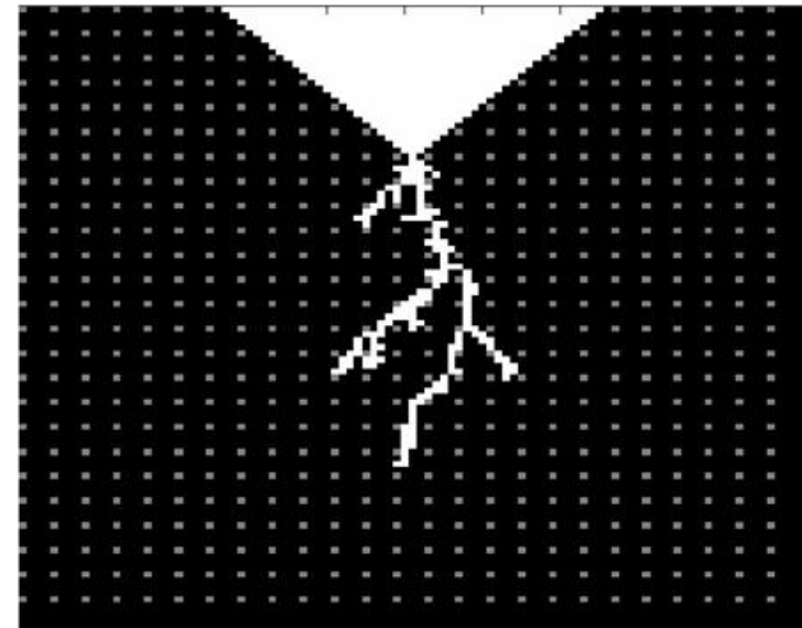
Fig. 5: Simulation with epoxy resin filled with \text{TiO}_2 nanoparticles (loading of 2 wt%, nanoparticle diameter 100 nm)
