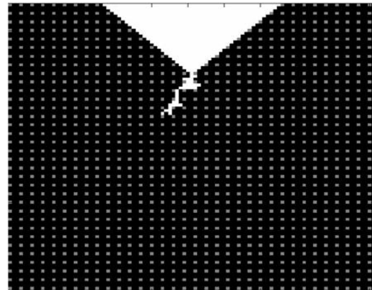
Fig. 6: Simulation with epoxy resin filled with \text{TiO}_2 nanoparticles (loading of 6 wt%, nanoparticle diameter 100 nm)
