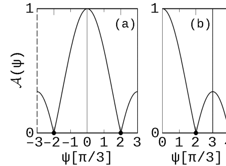
Fig. 12: ULA Array Factor A
