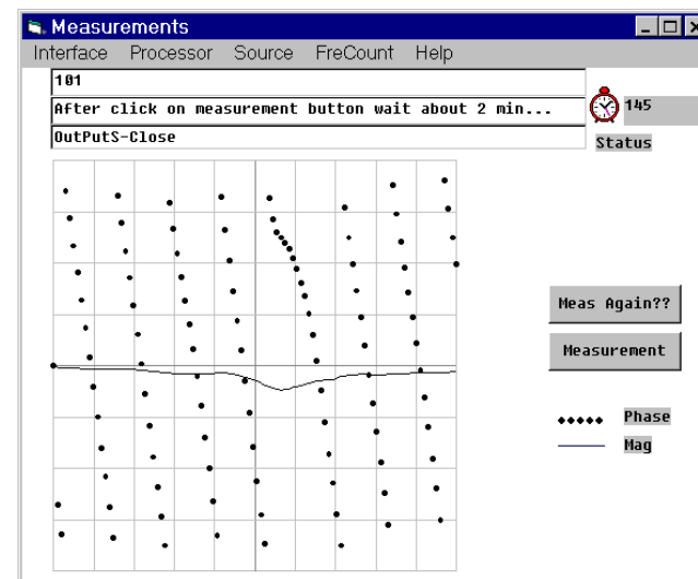
Fig. 11: [ANALYZE]-Output
