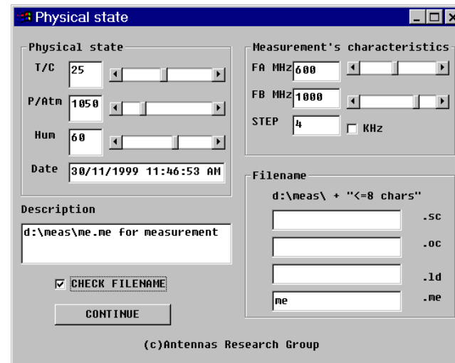
Fig.10: [ANALYZE]-Input
