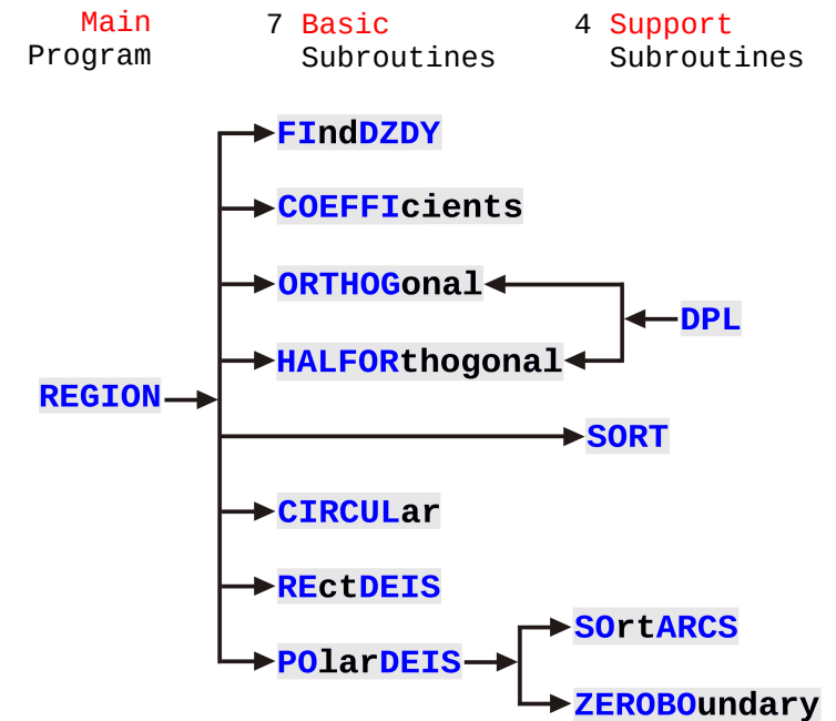
Fig. 7: REGION tool structure
